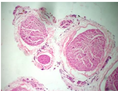
Figure 11. Acarbose + C. indica
