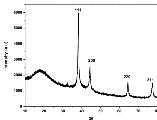
Figure 3. XRD patterns recorded for the silver nanoparticles synthesized from pappya extract
