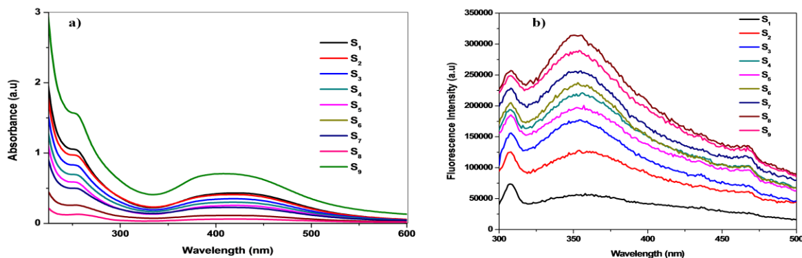
Figure 5. a) Absorption spectra of drug interacted nanoparticle samples (S 1 - S 9 ) was observed at 267nm and 420nm for drug and nanoparticles respectively, b) Emission spectra of drug interacted nanoparticle samples (S 1 - S 9 ) was observed at 350nm and 460 nm respectively.
