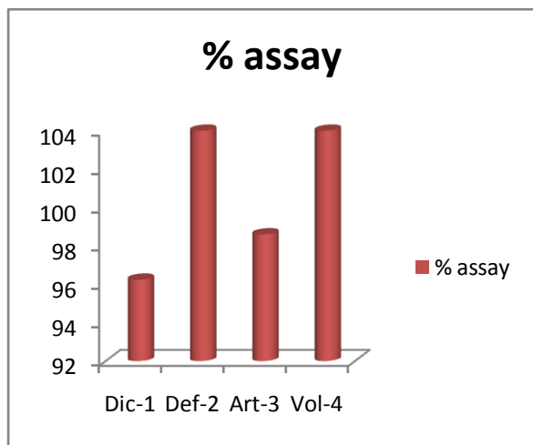
Figure 2 : % Assay of different brands of Diclofenac sodium
