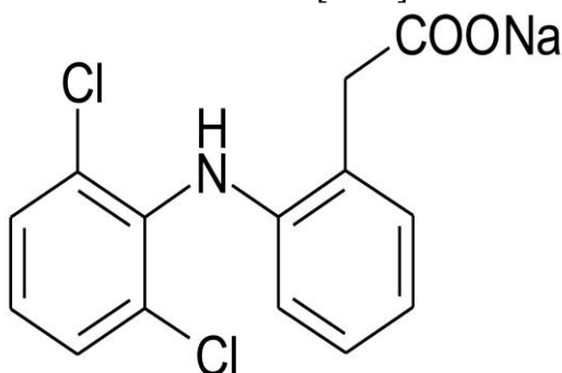
Figure 1: Structure of Diclofenac Sodium
