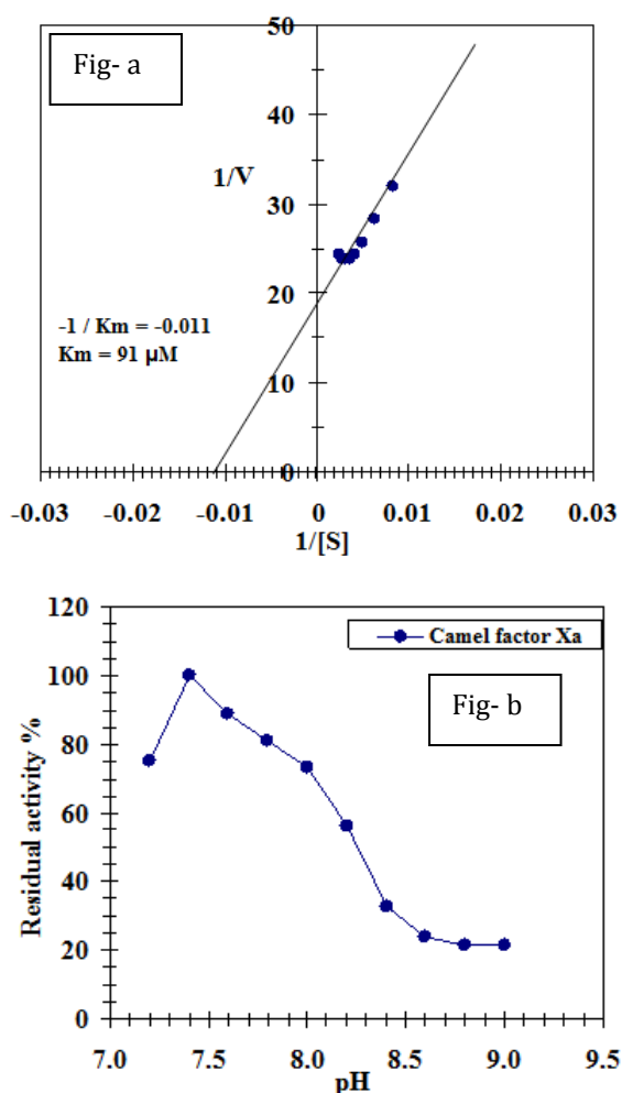
Figure 3. (a) Lineweaver-Burk plot for the reciprocal of the reaction velocity of the purified camel FXa (1/V) and substrate concentration (1/[S]). (b) Effect of pH on the purified camel FXa activity using N-Benzoyl-Ile-Glu-Gly-Arg-p-nitroanilide HCl as substrate in 0.05 M Tris-HCl buffer.
