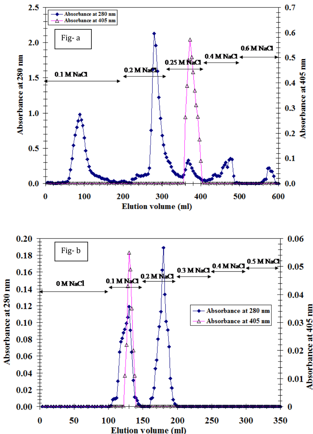
Figure 2. (a) A typical elution profile for the chromatography of barium adsorbate of camel plasma on a DEAE-cellulose column previously equilibrated with 0.025 M sodium citrate, pH 6.0, containing 0.1 M NaCl and 0.001M benzamidine HCl. (b) A typical elution profile for the chromatography of DEAE-cellulose pooled fractions on a column of heparin-agarose previously equilibrated with 0.02 M sodium citrate, pH 7.5, containing 0.001M benzamidine HCl.
