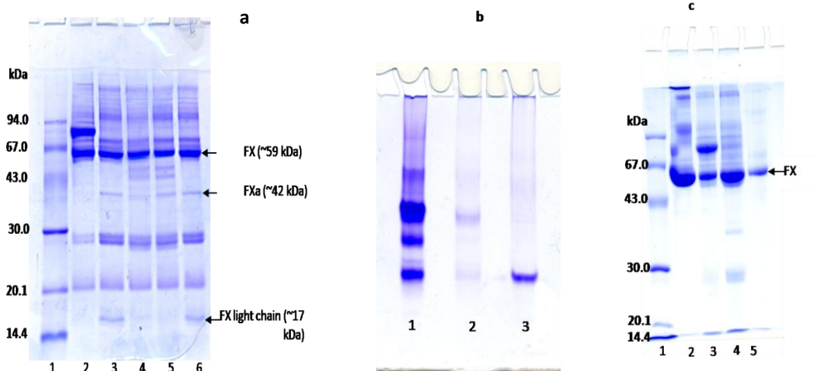
Figure 1. (a) 12% SDS PAGE analysis of barium adsorbate containing FX samples subjected to activation, (1) molecular weight markers, (2) sample before activation (3) activated sample with Cerastus cerastus viper venom (4) activated sample with Echus carinatus viper venom (5) activated sample with thromboplastin (1:40 w/w) (6) activated sample with thromboplastin (1:20 w/w). (b) Native 7% PAGE for purification steps of camel FX: (1) the barium adsorbate fraction, (2) DEAE-cellulose fraction, (3) heparin-agarose fraction. (c) 12% SDS PAGE (1) molecular weight markers, (2) plasma, (3) the barium adsorbate fraction, (4) DEAE-cellulose fraction, (5) heparin-agarose fraction.
