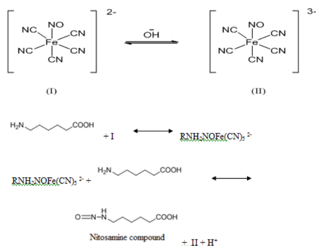
Scheme 1. Proposed pathway for ACA-SNP reaction
