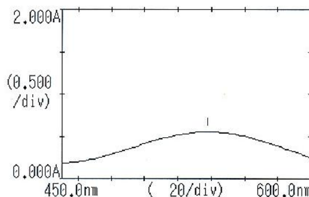
Figure 2. UV/VIS spectrum of the ACA-SNP complex.
